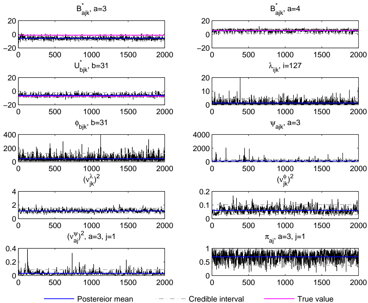
Trace plot, j=1, k=7 , DE data, simulation run 7
