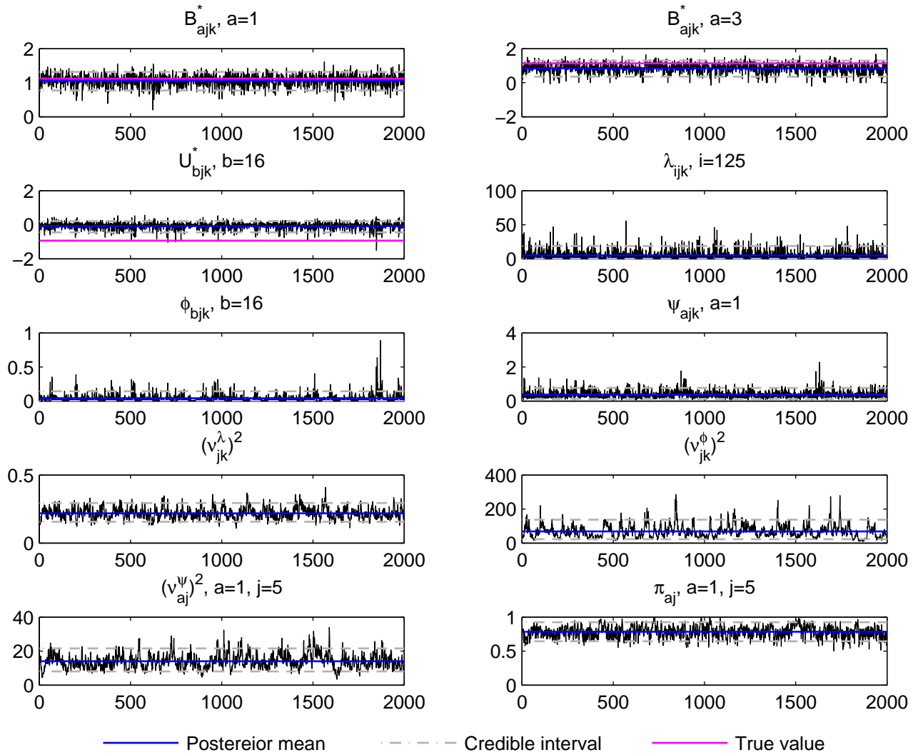
Trace plot, j=5, k=3, t_j data, simulation run 7
