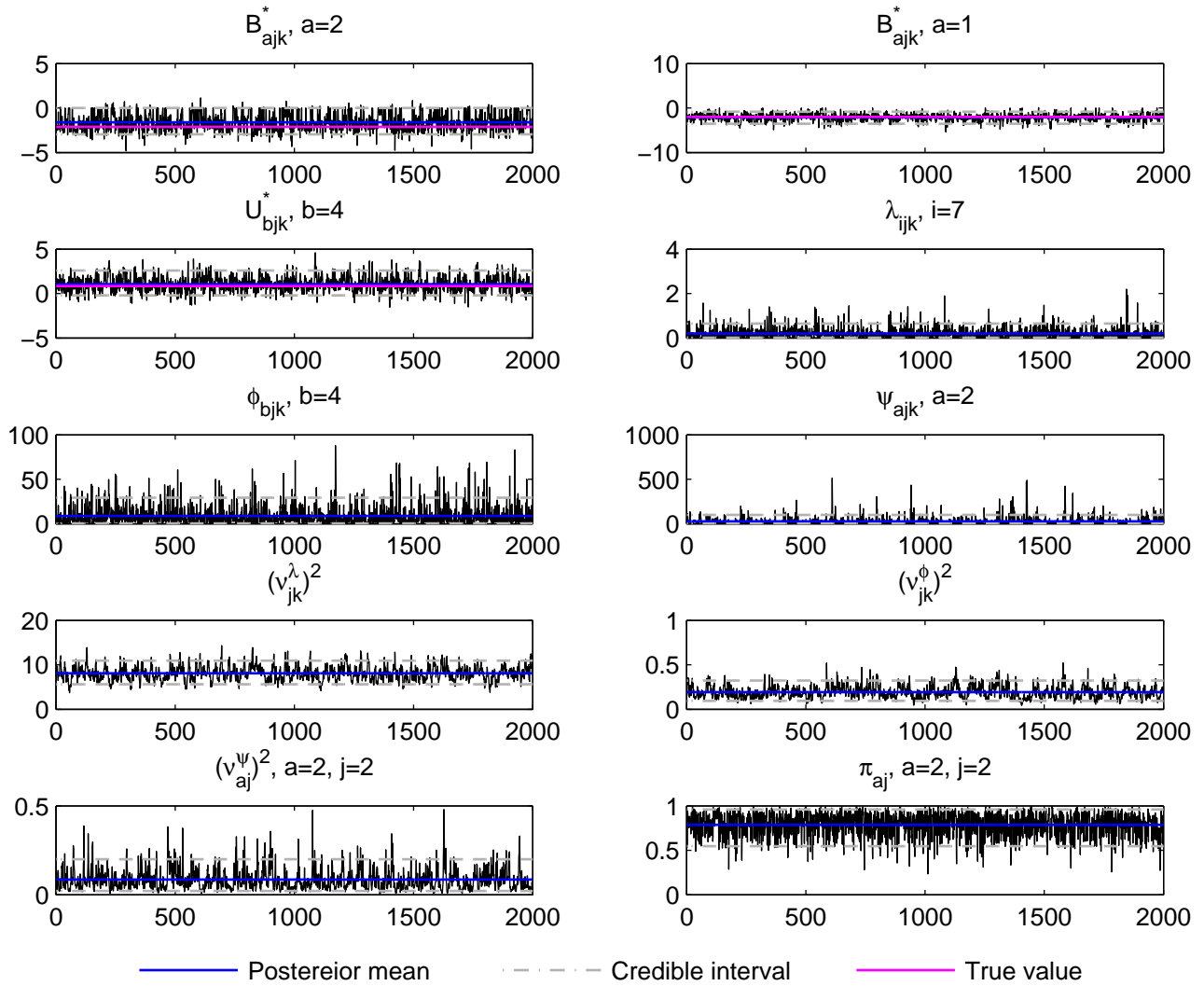
Trace plot, j=2, k=4, t_2 data, simulation run 7
