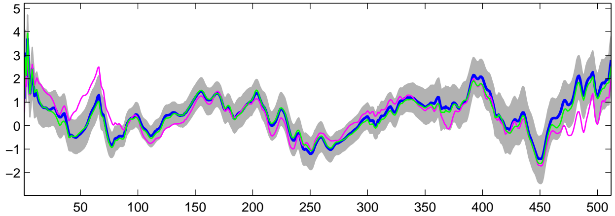
Estimated U_{10}(t) using G-WFMM: DE data, run 7
