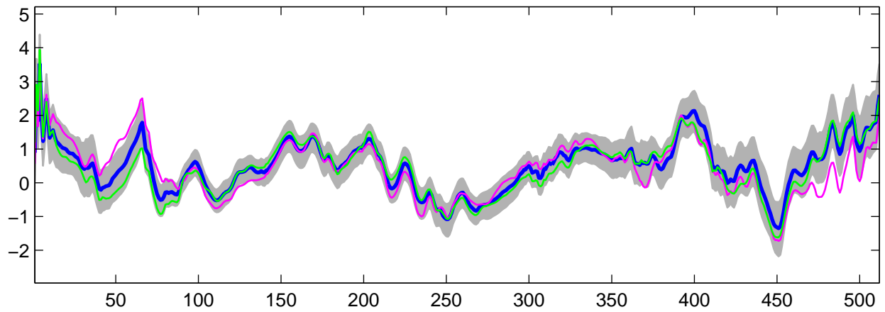
Estimated U_{10}(t) using R-WFMM: DE data, run 7
