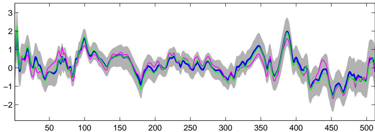
Estimated U_{10}(t) using G-WFMM: Normal data, run 7
