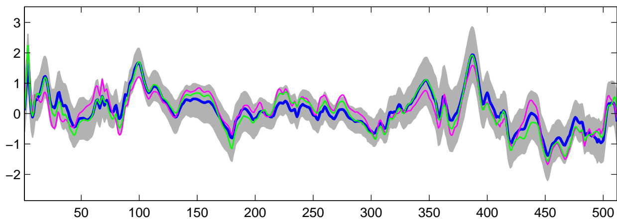
Estimated U_{10}(t) using R-WFMM: Normal data, run 7
