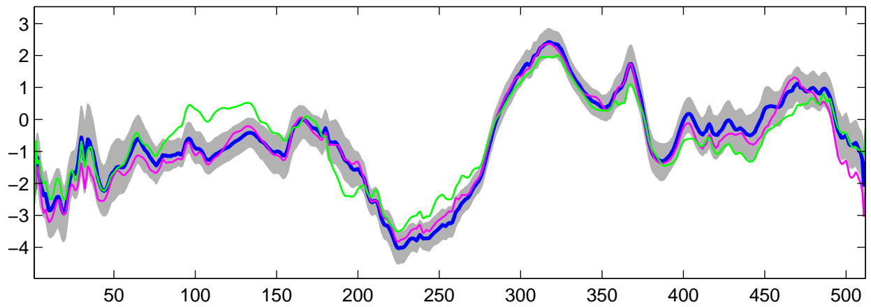
Estimated U_{10}(t) using R-WFMM: t_2 data, run 7
