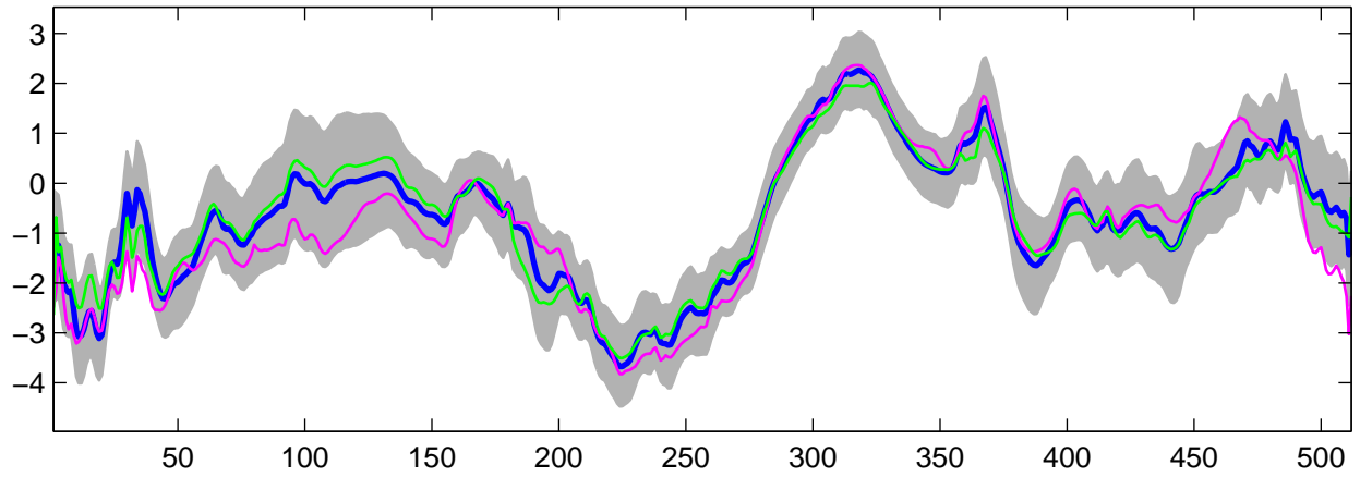
Estimated U_{10}(t) using G-WFMM: t_2 data, run 7
