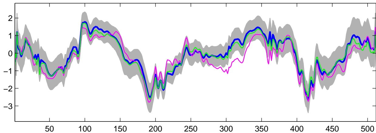
Estimated U_{11}(t) using G-WFMM: Normal data, run 7
