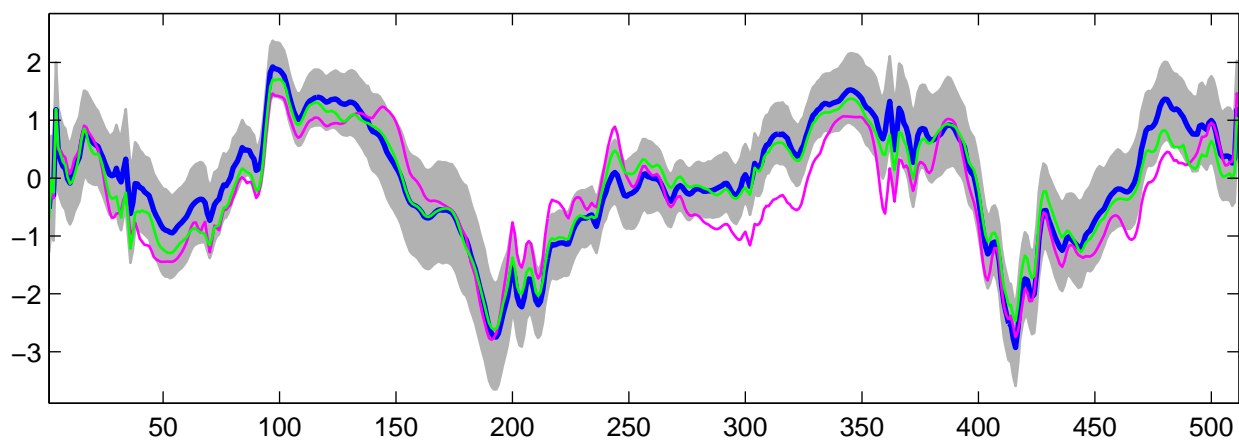
Estimated U_{11}(t) using R-WFMM: Normal data, run 7
