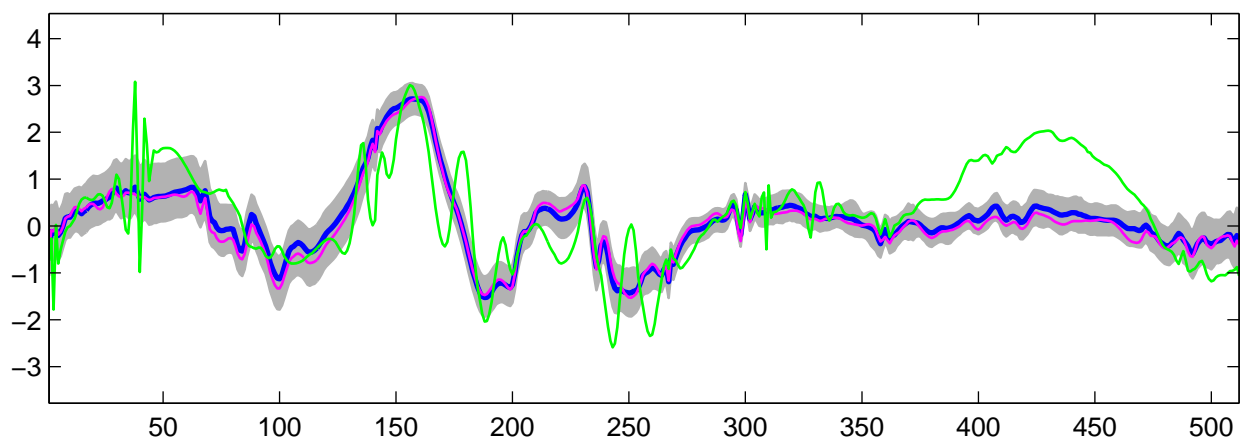
Estimated U_{11}(t) using R-WFMM: t_1 data, run 7
