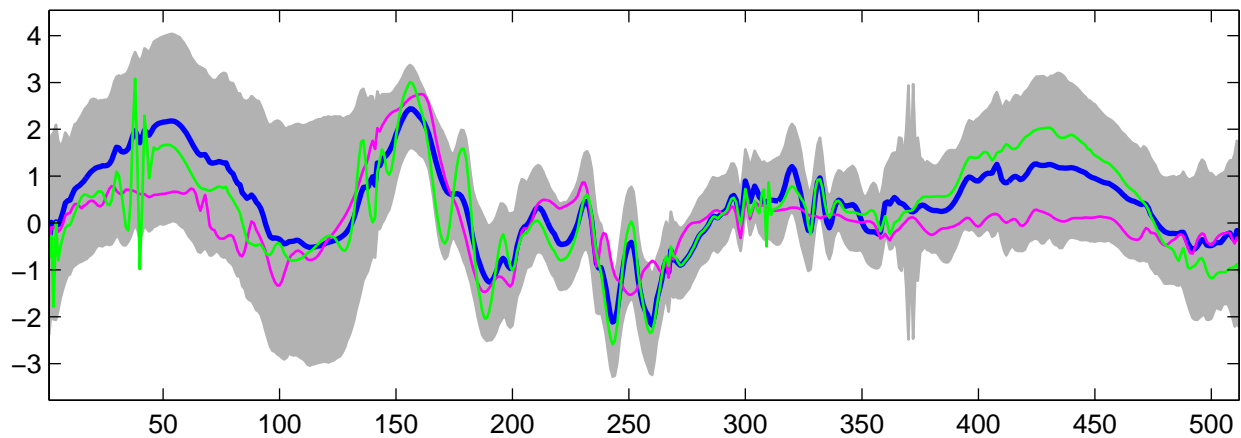
Estimated U_{11}(t) using G-WFMM: t_1 data, run 7
