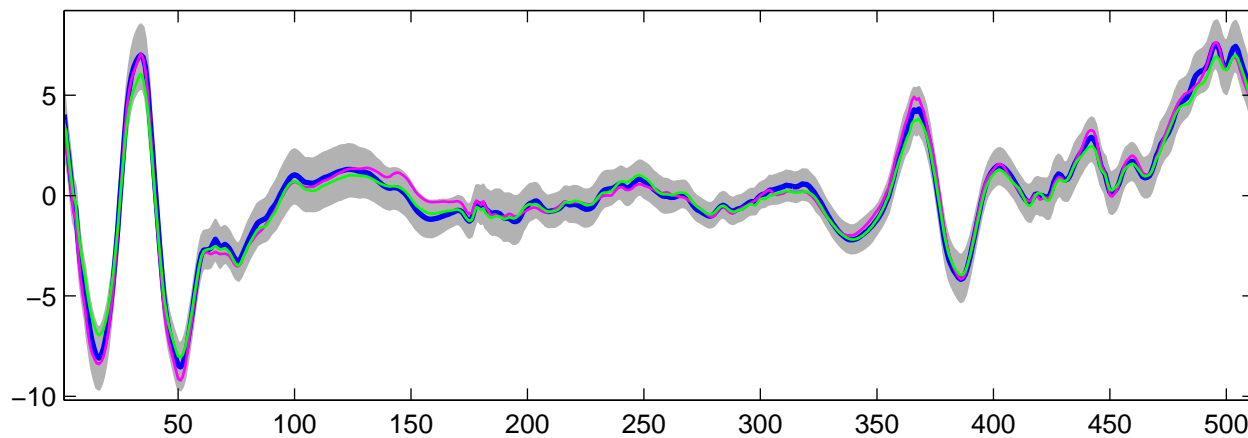
Estimated U_{11}(t) using G-WFMM: t_2 data, run 7
