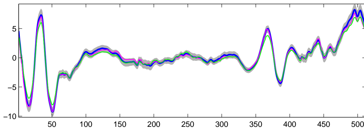
Estimated U_{11}(t) using R-WFMM: t_2 data, run 7
