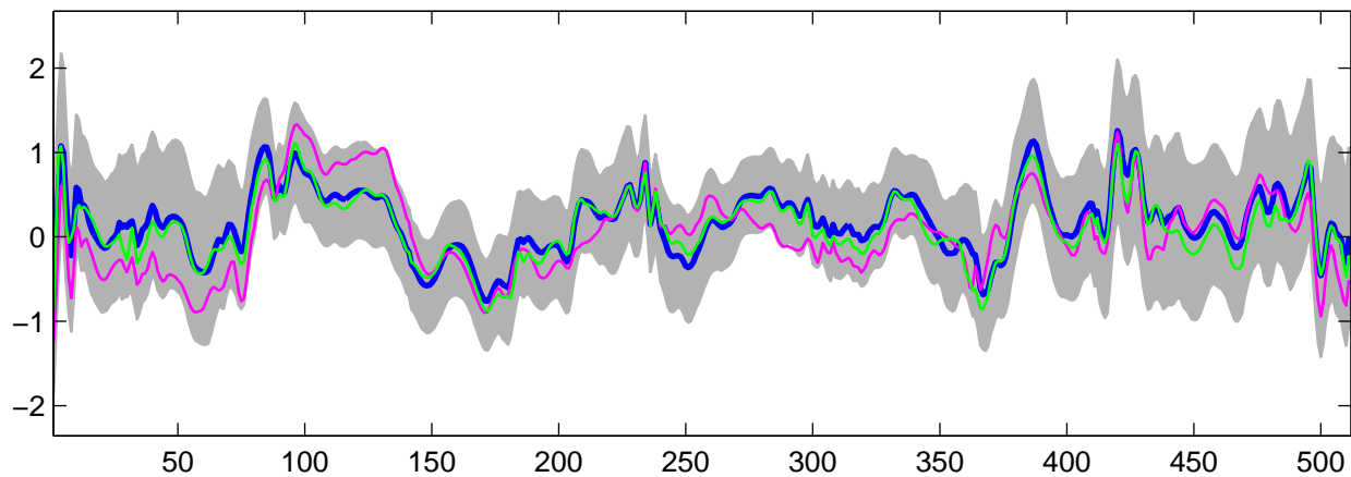
Estimated U_{11}(t) using G-WFMM: t_3 data, run 7
