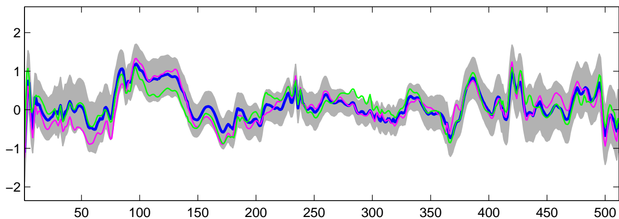
Estimated U_{11}(t) using R-WFMM: t_3 data, run 7
