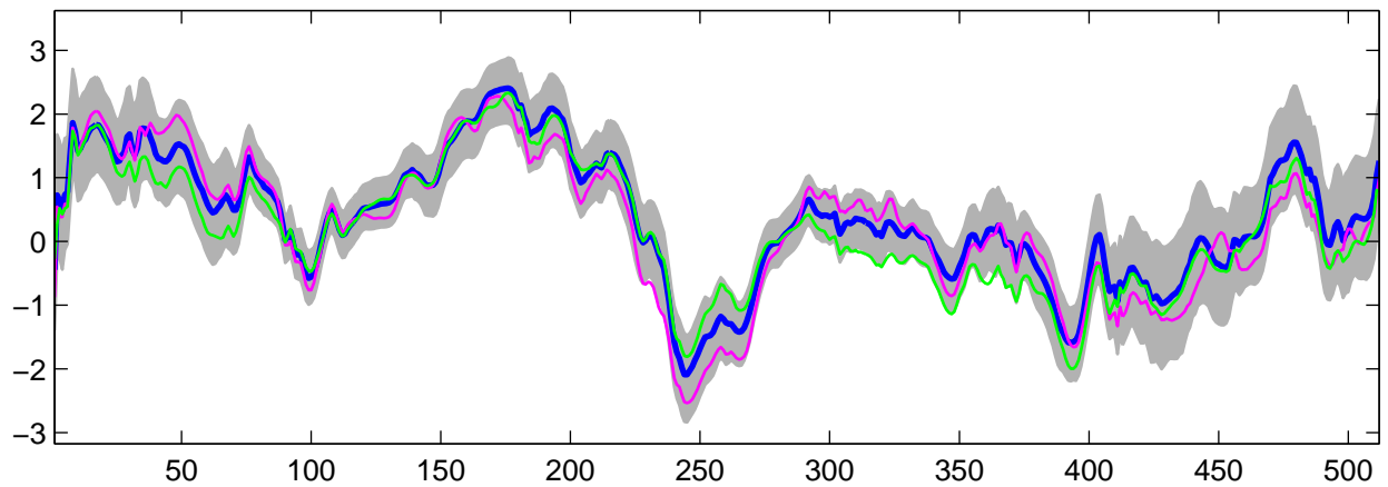
Estimated U_{12}(t) using R-WFMM: DE data, run 7
