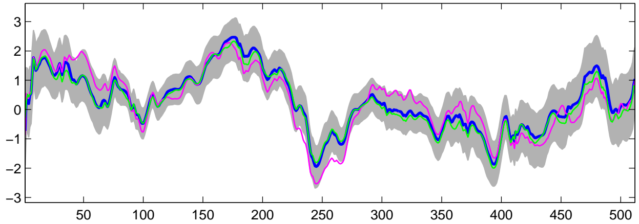
Estimated U_{12}(t) using G-WFMM: DE data, run 7
