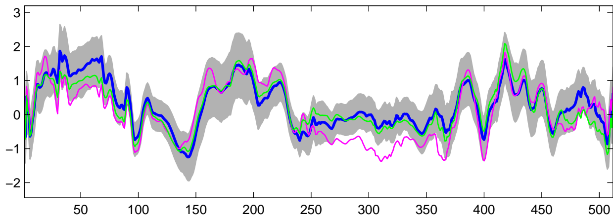
Estimated U_{12}(t) using R-WFMM: Normal data, run 7
