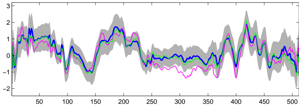
Estimated U_{12}(t) using G-WFMM: Normal data, run 7
