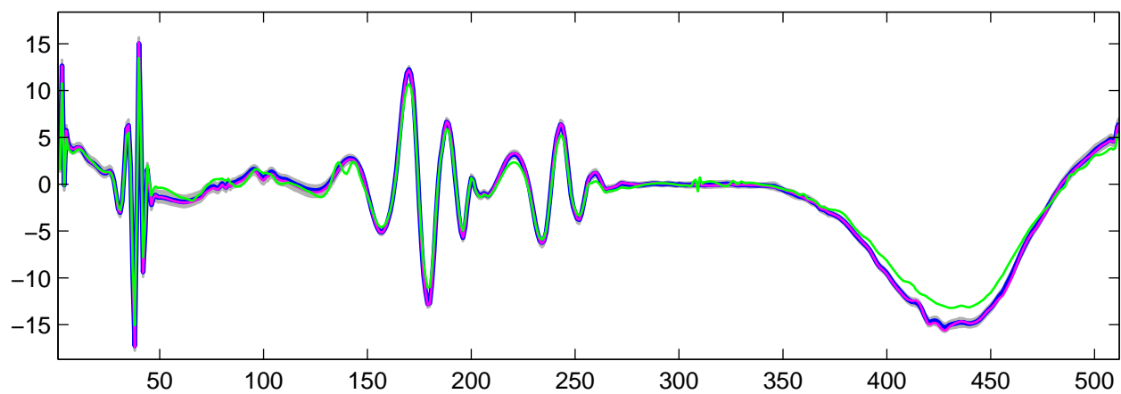
Estimated U_{12}(t) using R-WFMM: t_1 data, run 7
