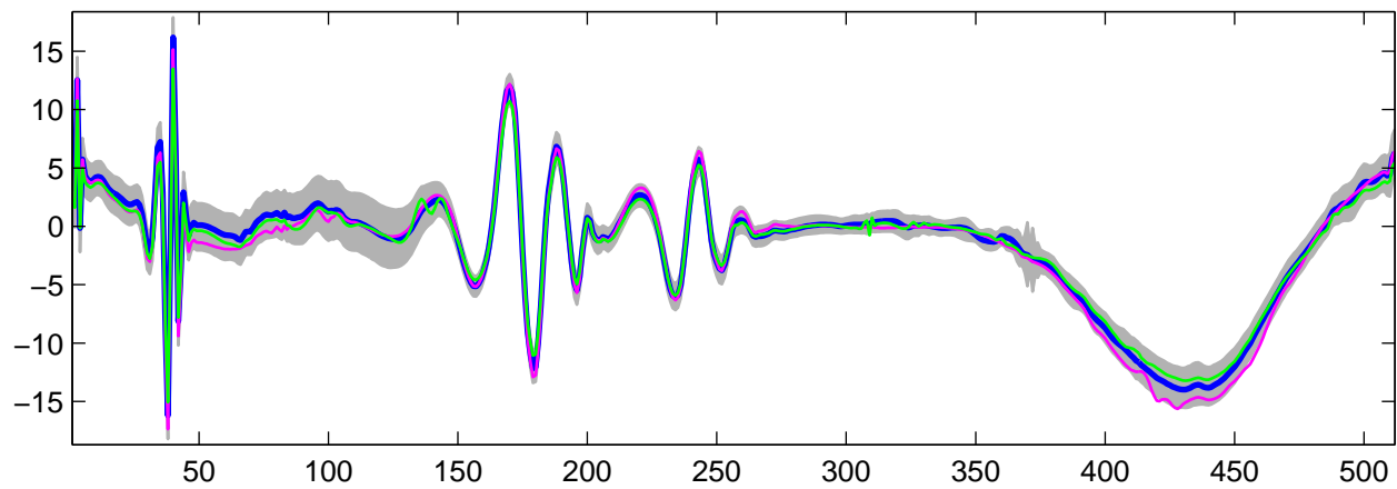
Estimated U_{12}(t) using G-WFMM: t_1 data, run 7
