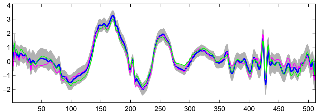
Estimated U_{12}(t) using R-WFMM: t_3 data, run 7
