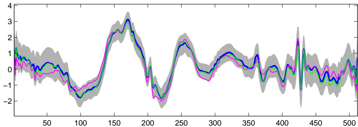
Estimated U_{12}(t) using G-WFMM: t_3 data, run 7
