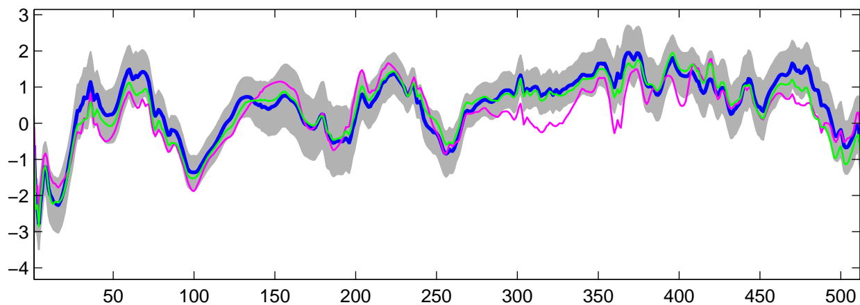
Estimated U_{13}(t) using R-WFMM: Normal data, run 7
