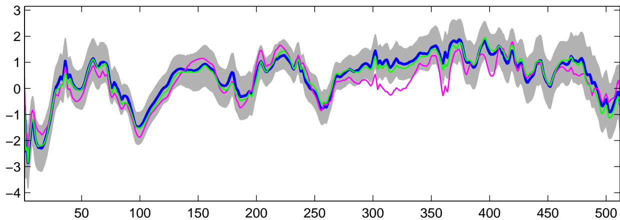
Estimated U_{13}(t) using G-WFMM: Normal data, run 7
