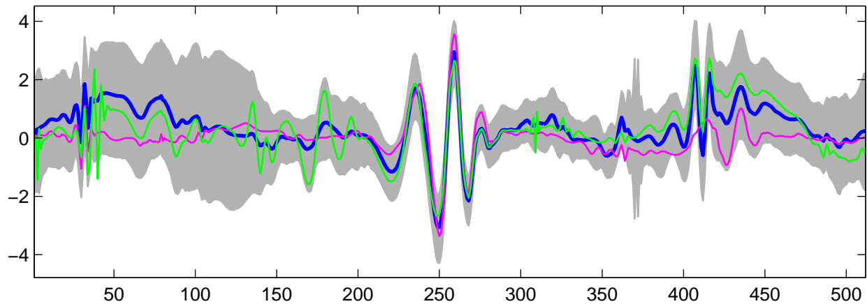
Estimated U_{13}(t) using G-WFMM: t_1 data, run 7
