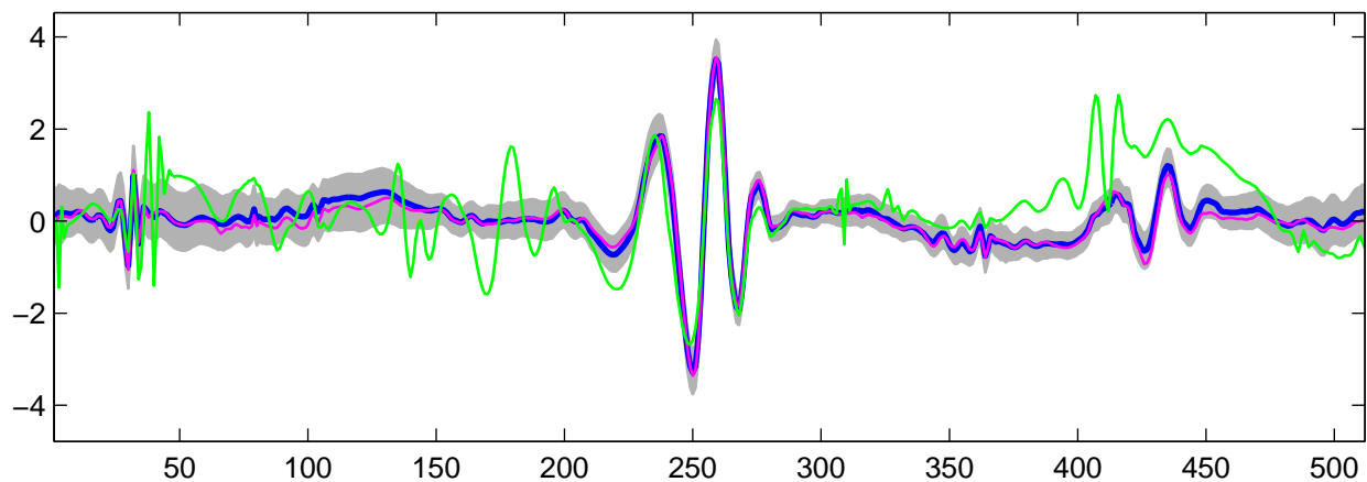
Estimated U_{13}(t) using R-WFMM: t_1 data, run 7
