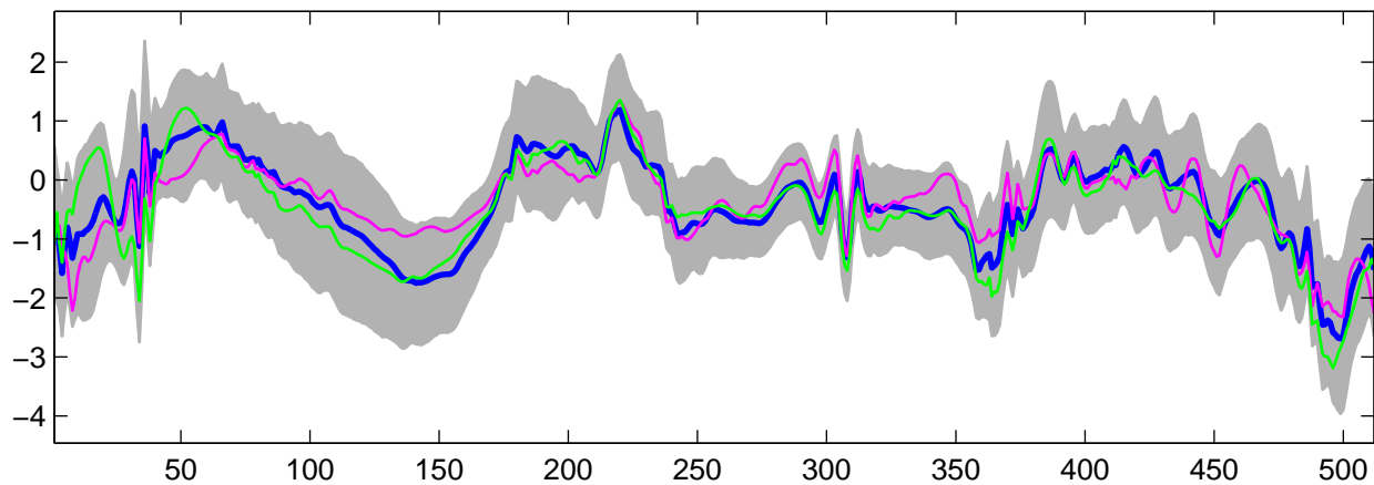
Estimated U_{13}(t) using G-WFMM: t_2 data, run 7
