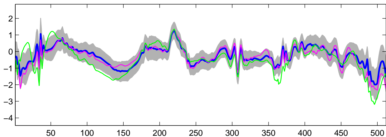
Estimated U_{13}(t) using R-WFMM: t_2 data, run 7
