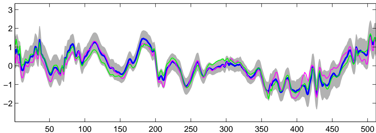
Estimated U_{13}(t) using R-WFMM: t_3 data, run 7
