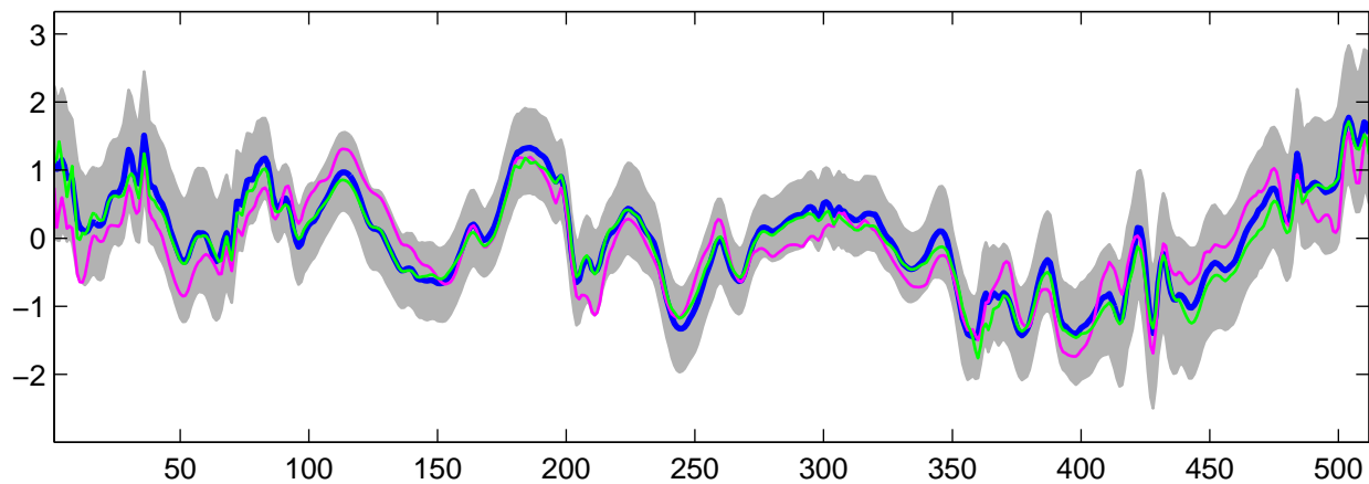
Estimated U_{13}(t) using G-WFMM: t_3 data, run 7
