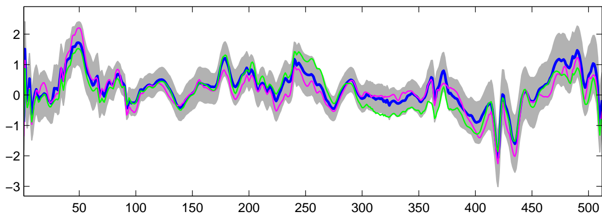
Estimated U_{14}(t) using R-WFMM: DE data, run 7
