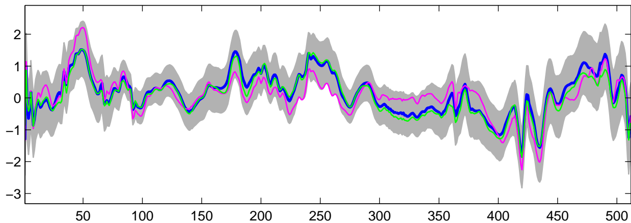
Estimated U_{14}(t) using G-WFMM: DE data, run 7
