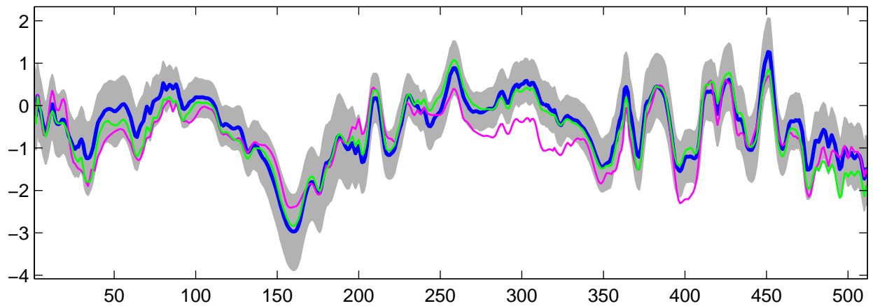
Estimated U_{14}(t) using R-WFMM: Normal data, run 7
