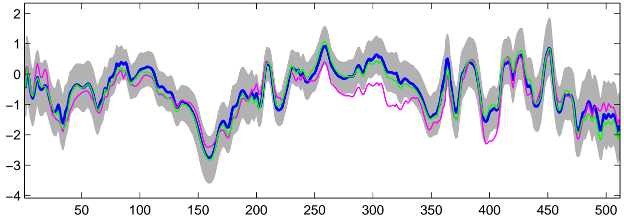
Estimated U_{14}(t) using G-WFMM: Normal data, run 7
