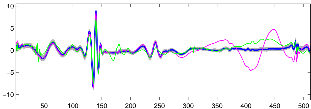
Estimated U_{14}(t) using R-WFMM: t_1 data, run 7
