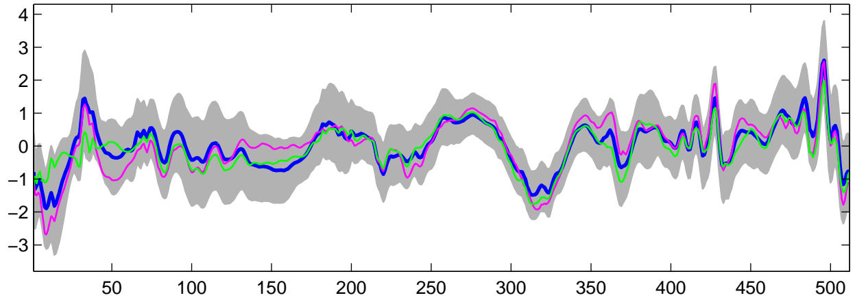
Estimated U_{14}(t) using G-WFMM: t_2 data, run 7
