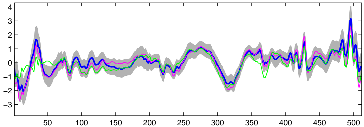
Estimated U_{14}(t) using R-WFMM: t_2 data, run 7
