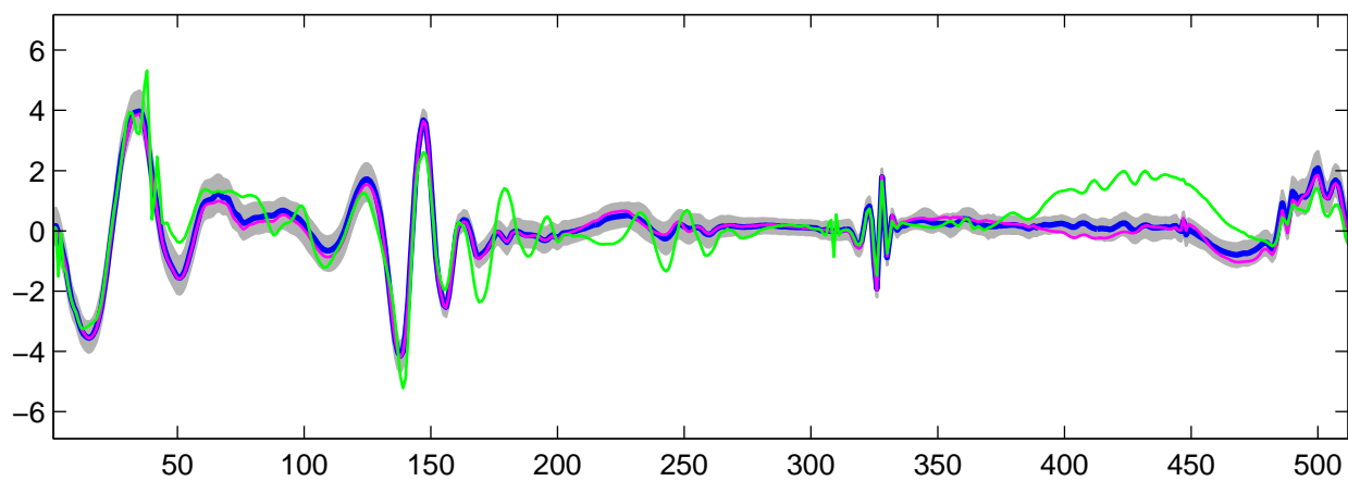
Estimated U_{15}(t) using R-WFMM: t_1 data, run 7
