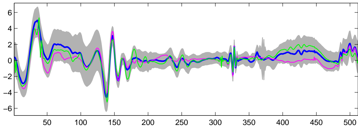
Estimated U_{15}(t) using G-WFMM: t_1 data, run 7
