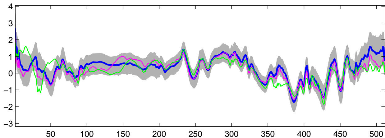
Estimated U_{15}(t) using R-WFMM: t_2 data, run 7
