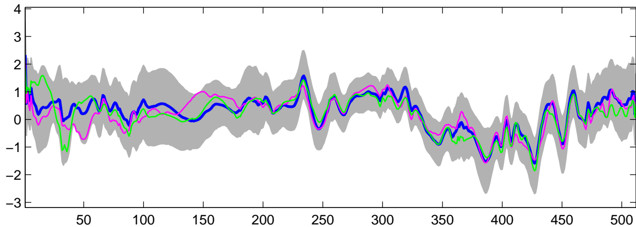
Estimated U_{15}(t) using G-WFMM: t_2 data, run 7
