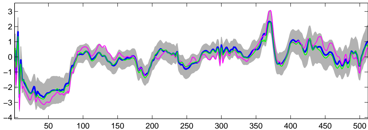
Estimated U_{15}(t) using G-WFMM: t_3 data, run 7
