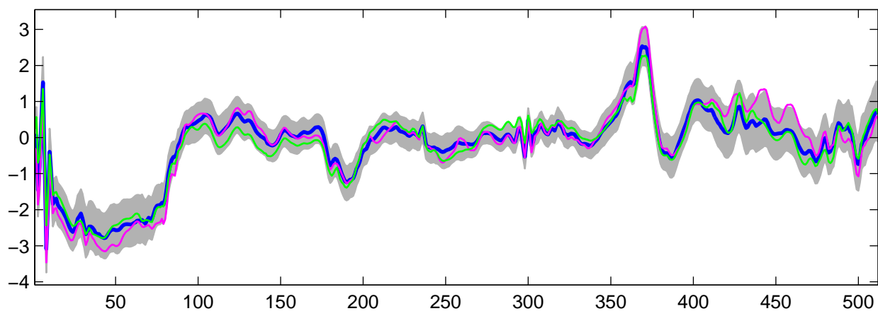
Estimated U_{15}(t) using R-WFMM: t_3 data, run 7
