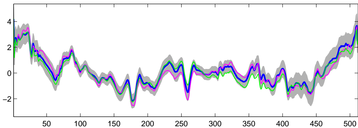
Estimated U_{16}(t) using R-WFMM: DE data, run 7
