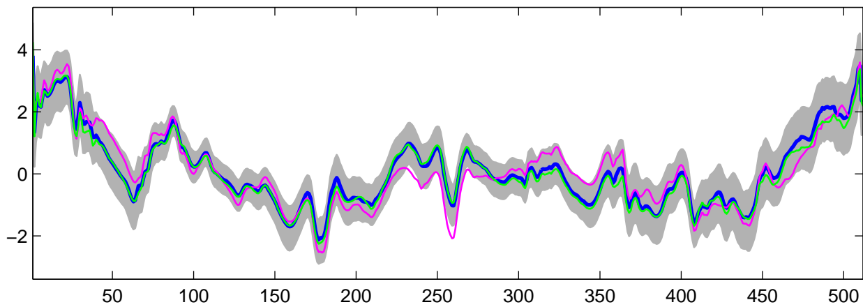
Estimated U_{16}(t) using G-WFMM: DE data, run 7
