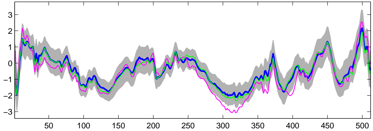
Estimated U_{16}(t) using G-WFMM: Normal data, run 7
