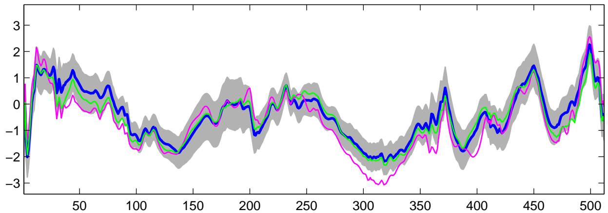
Estimated U_{16}(t) using R-WFMM: Normal data, run 7
