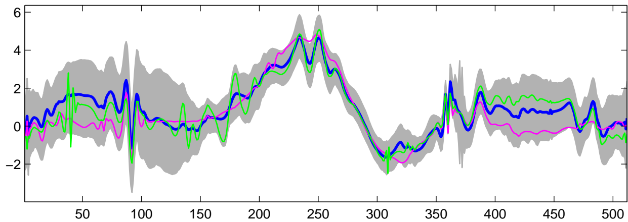
Estimated U_{16}(t) using G-WFMM: t_1 data, run 7
