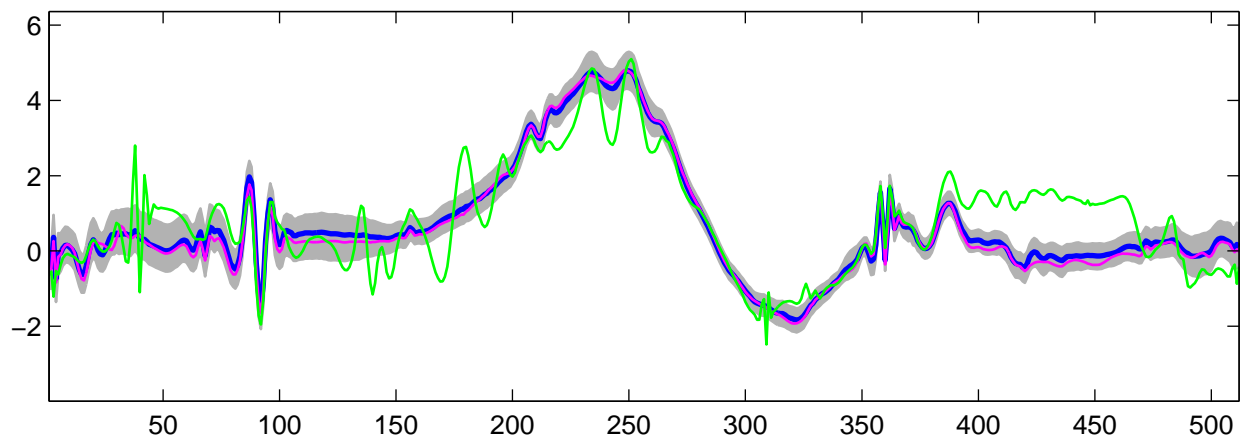
Estimated U_{16}(t) using R-WFMM: t_1 data, run 7
