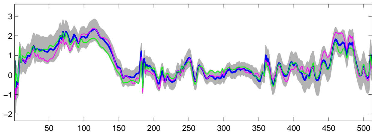
Estimated U_{16}(t) using R-WFMM: t_3 data, run 7
