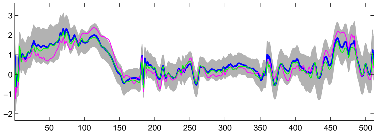
Estimated U_{16}(t) using G-WFMM: t_3 data, run 7
