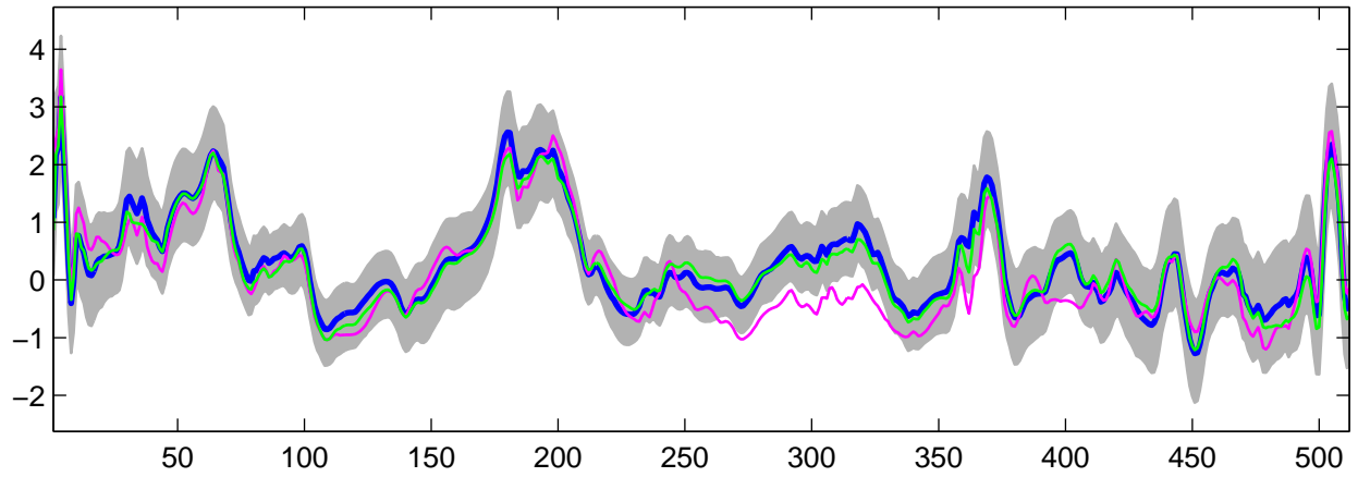
Estimated U_{18}(t) using G-WFMM: Normal data, run 7
