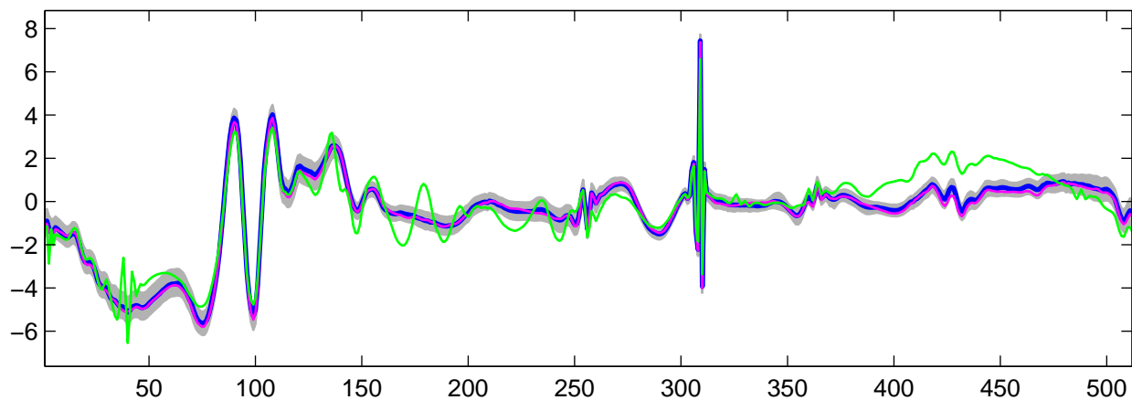
Estimated U_{18}(t) using R-WFMM: t_1 data, run 7
