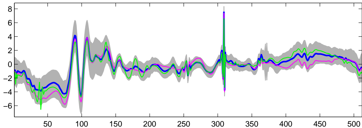
Estimated U_{18}(t) using G-WFMM: t_1 data, run 7
