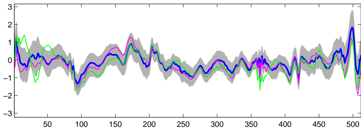
Estimated U_{18}(t) using R-WFMM: t_2 data, run 7
