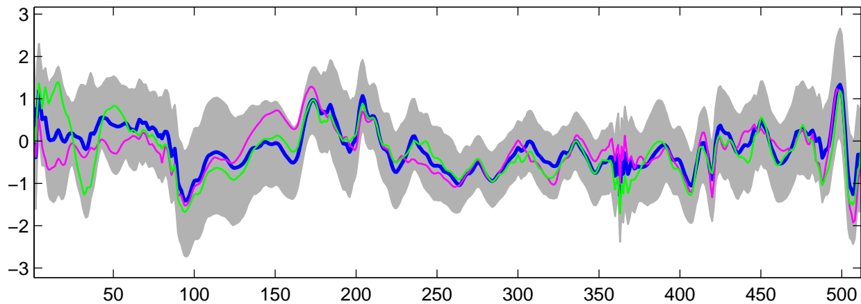
Estimated U_{18}(t) using G-WFMM: t_2 data, run 7
