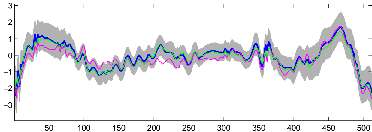
Estimated U_{18}(t) using G-WFMM: t_3 data, run 7
