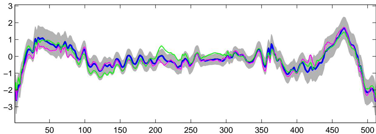
Estimated U_{18}(t) using R-WFMM: t_3 data, run 7
