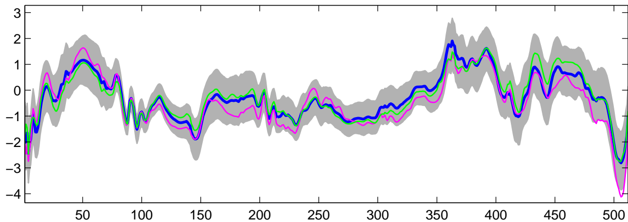
Estimated U_{19}(t) using G-WFMM: DE data, run 7
