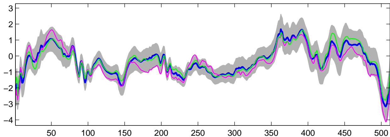
Estimated U_{19}(t) using R-WFMM: DE data, run 7
