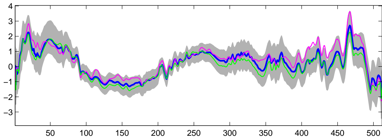
Estimated U_{19}(t) using R-WFMM: Normal data, run 7
