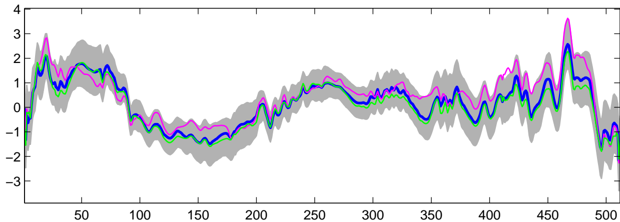
Estimated U_{19}(t) using G-WFMM: Normal data, run 7
