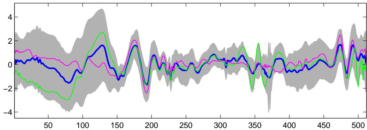
Estimated U_{19}(t) using G-WFMM: t_1 data, run 7
