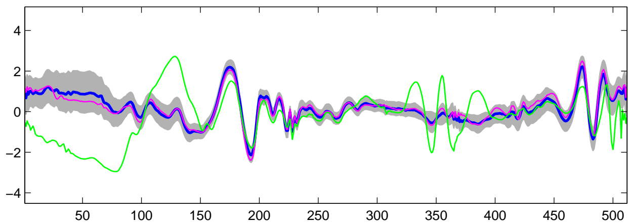
Estimated U_{19}(t) using R-WFMM: t_1 data, run 7
