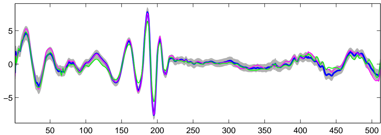
Estimated U_{19}(t) using R-WFMM: t_2 data, run 7
