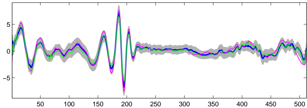
Estimated U_{19}(t) using G-WFMM: t_2 data, run 7
