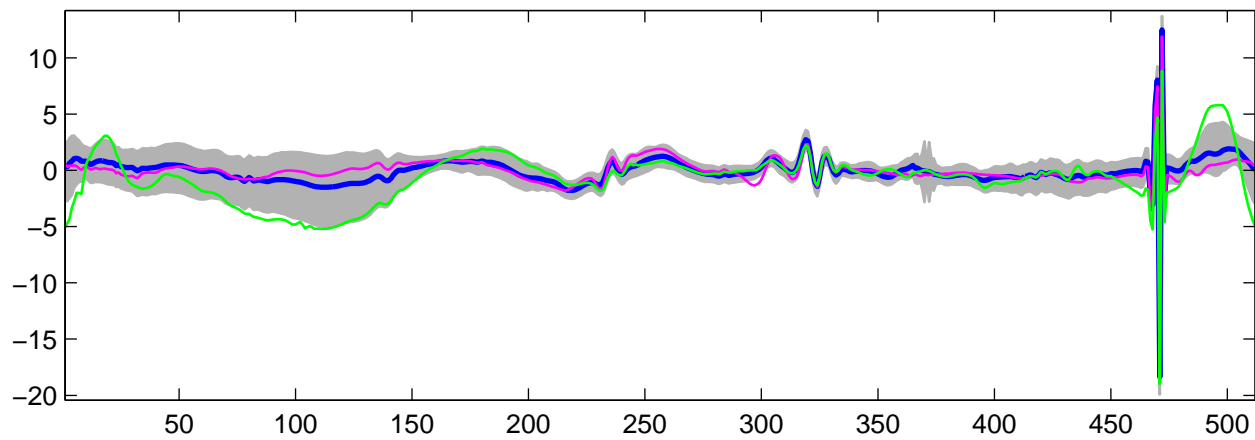
Estimated U_1(t) using G-WFMM: t_1 data, run 7
