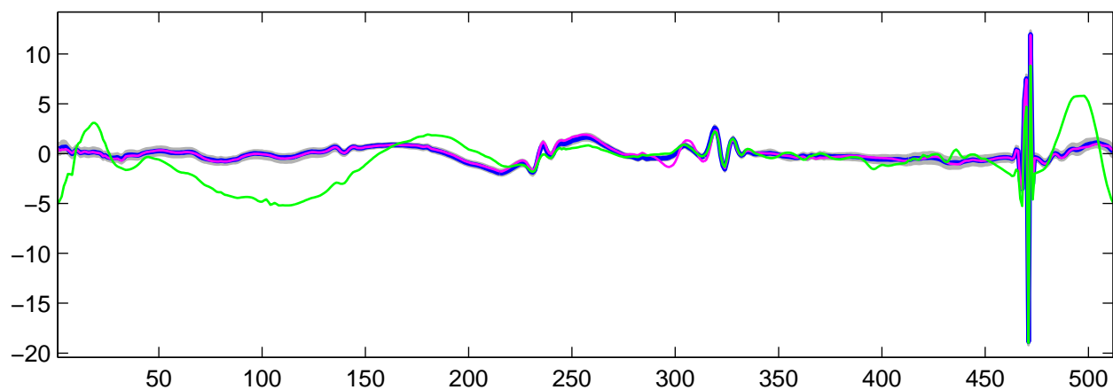
Estimated U_1(t) using R-WFMM: t_1 data, run 7
