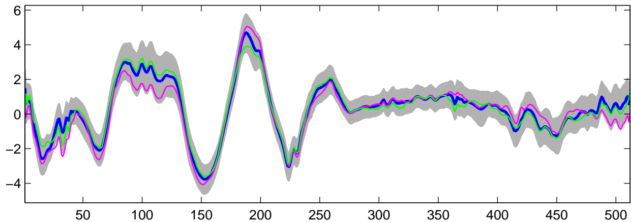
Estimated U_1(t) using G-WFMM: t_2 data, run 7
