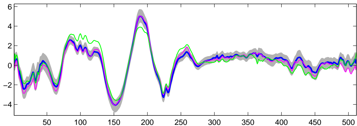
Estimated U_1(t) using R-WFMM: t_2 data, run 7
