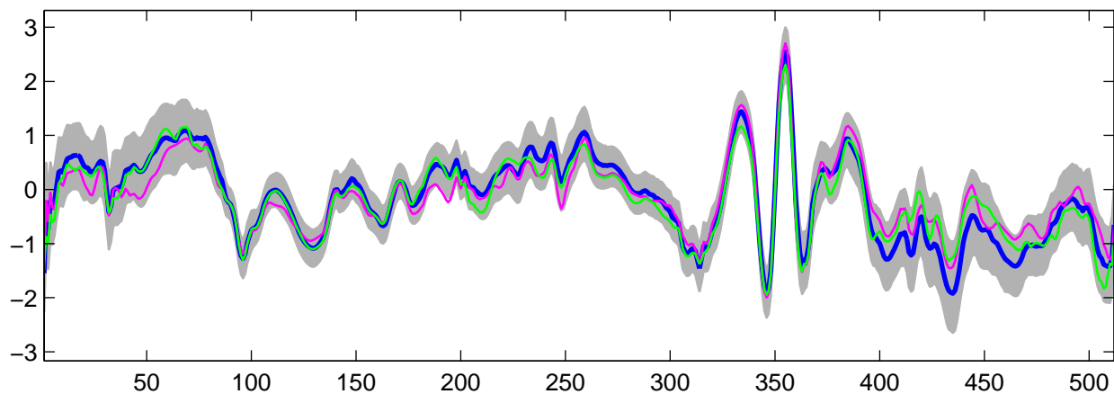
Estimated U_1(t) using R-WFMM: t_3 data, run 7
