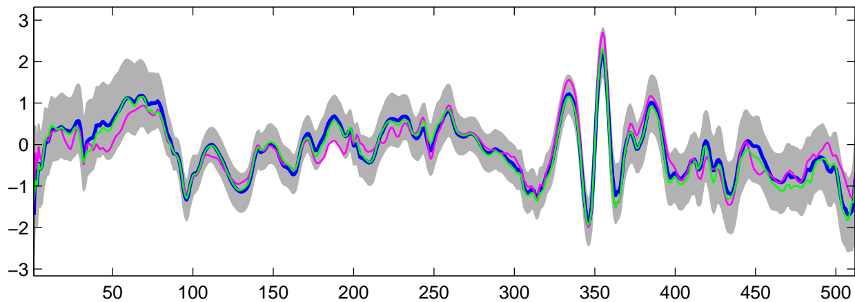
Estimated U_1(t) using G-WFMM: t_3 data, run 7
