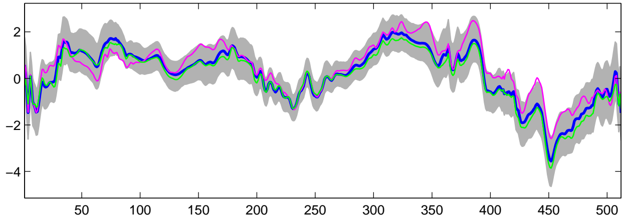
Estimated U_{20}(t) using G-WFMM: Normal data, run 7
