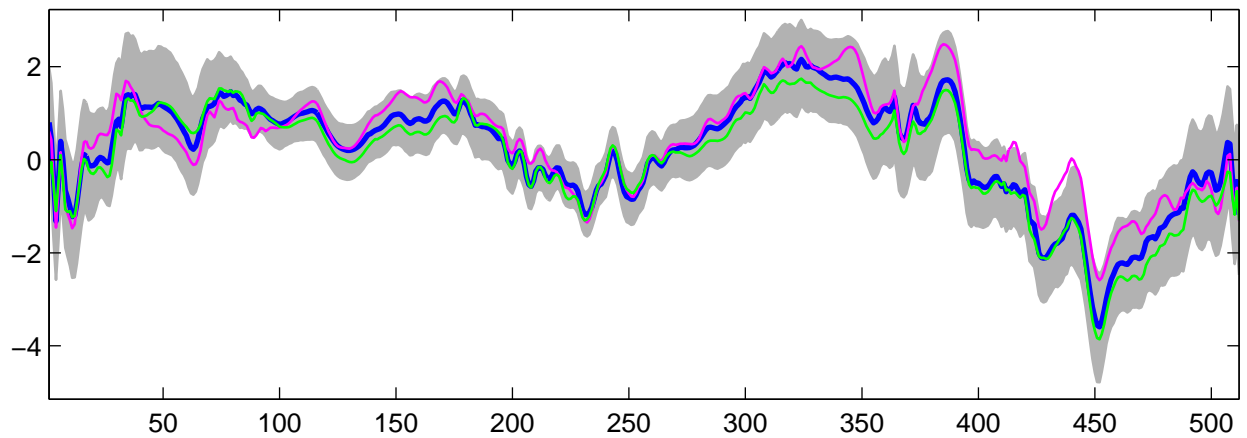
Estimated U_{20}(t) using R-WFMM: Normal data, run 7
