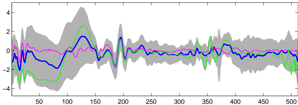
Estimated U_{20}(t) using G-WFMM: t_1 data, run 7
