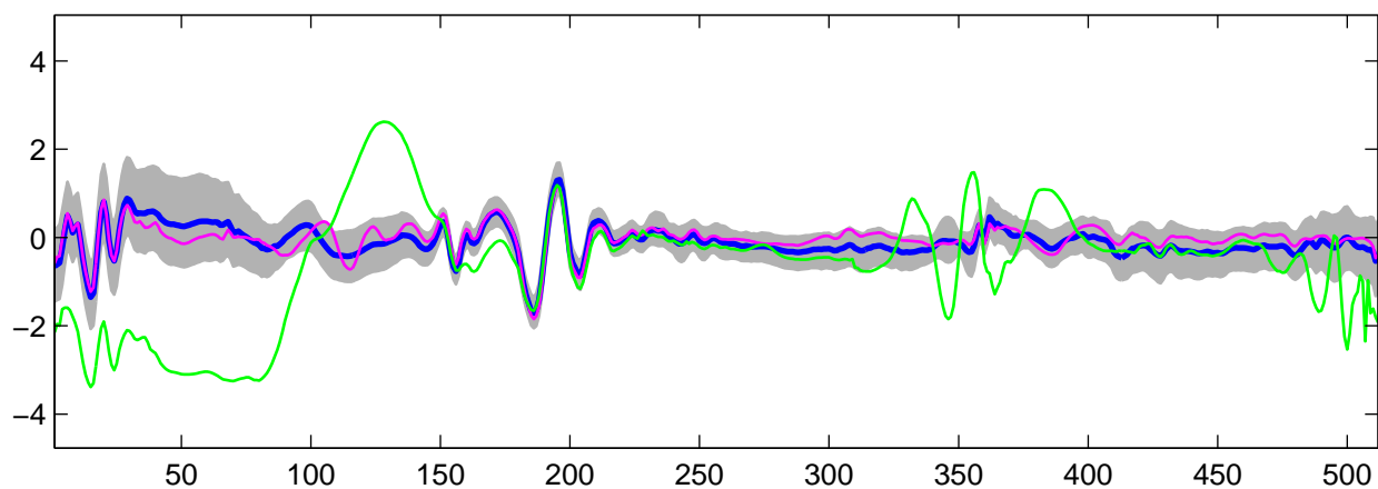
Estimated U_{20}(t) using R-WFMM: t_1 data, run 7
