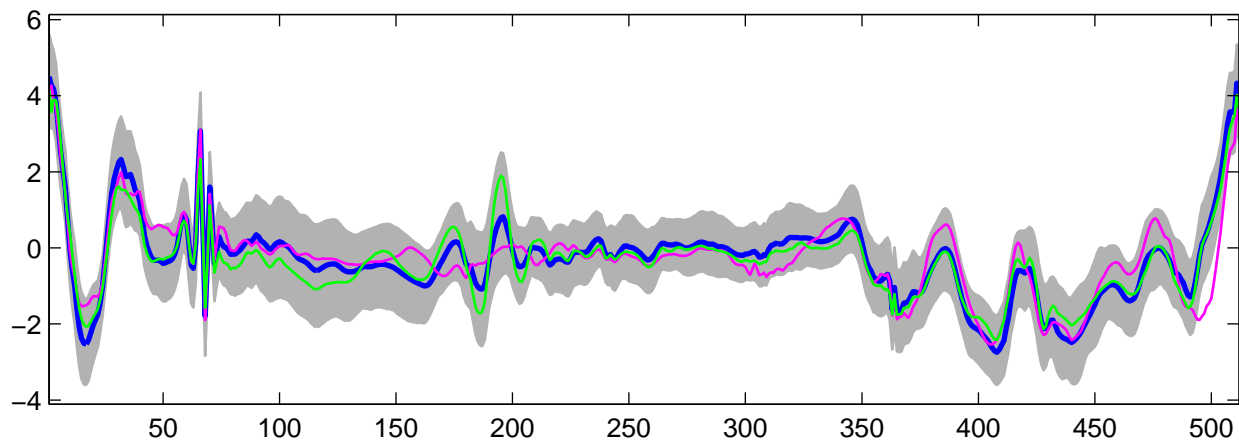
Estimated U_{20}(t) using G-WFMM: t_2 data, run 7
