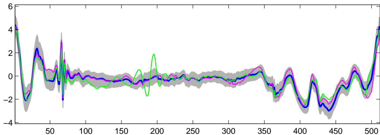
Estimated U_{20}(t) using R-WFMM: t_2 data, run 7
