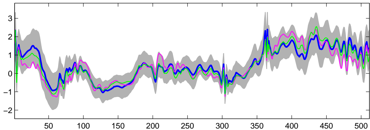
Estimated U_{20}(t) using G-WFMM: t_3 data, run 7
