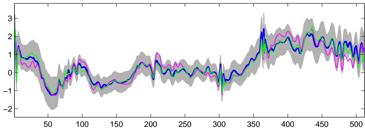
Estimated U_{20}(t) using R-WFMM: t_3 data, run 7
