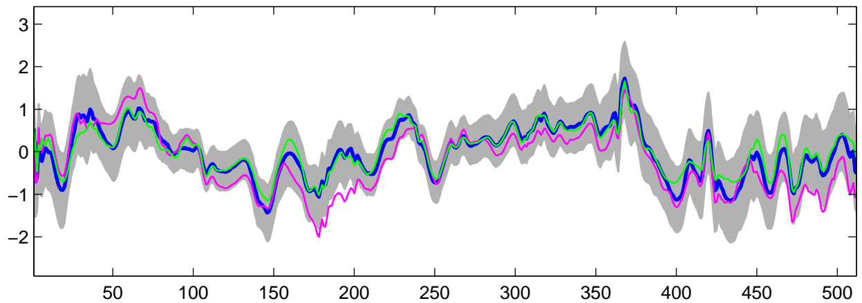
Estimated U_{21}(t) using R-WFMM: DE data, run 7
