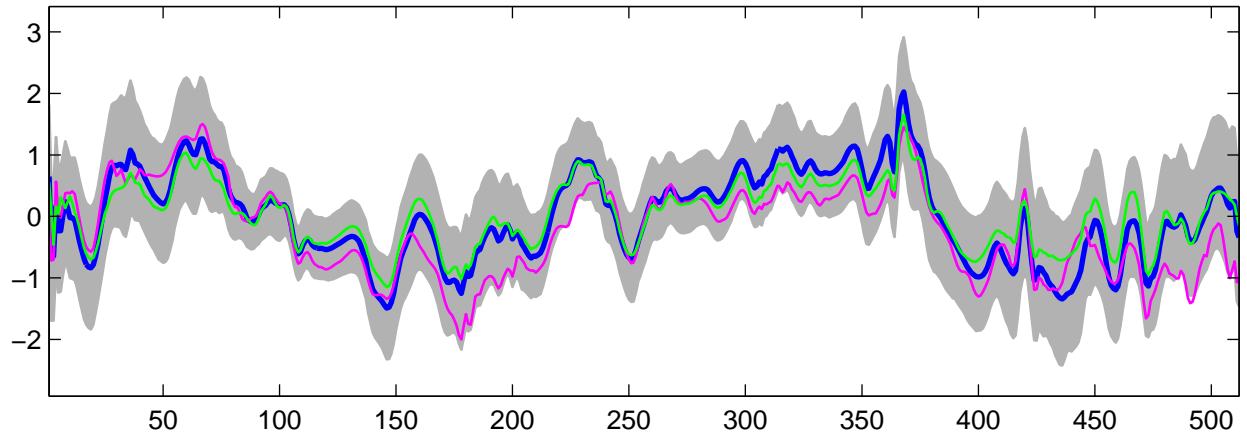
Estimated U_{21}(t) using G-WFMM: DE data, run 7
