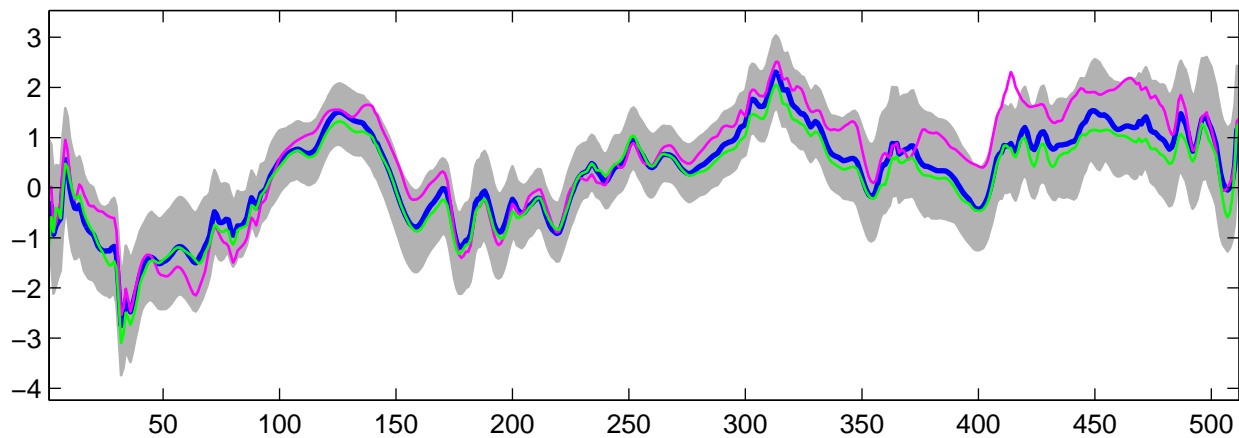
Estimated U_{21}(t) using G-WFMM: Normal data, run 7
