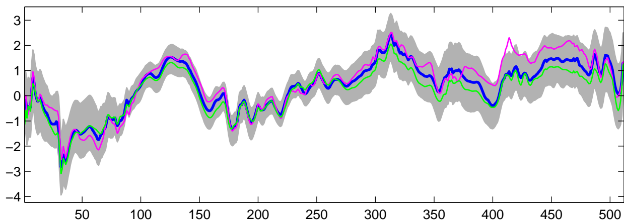
Estimated U_{21}(t) using R-WFMM: Normal data, run 7
