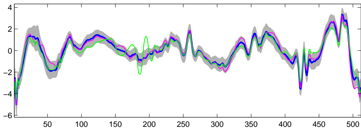
Estimated U_{21}(t) using R-WFMM: t_2 data, run 7
