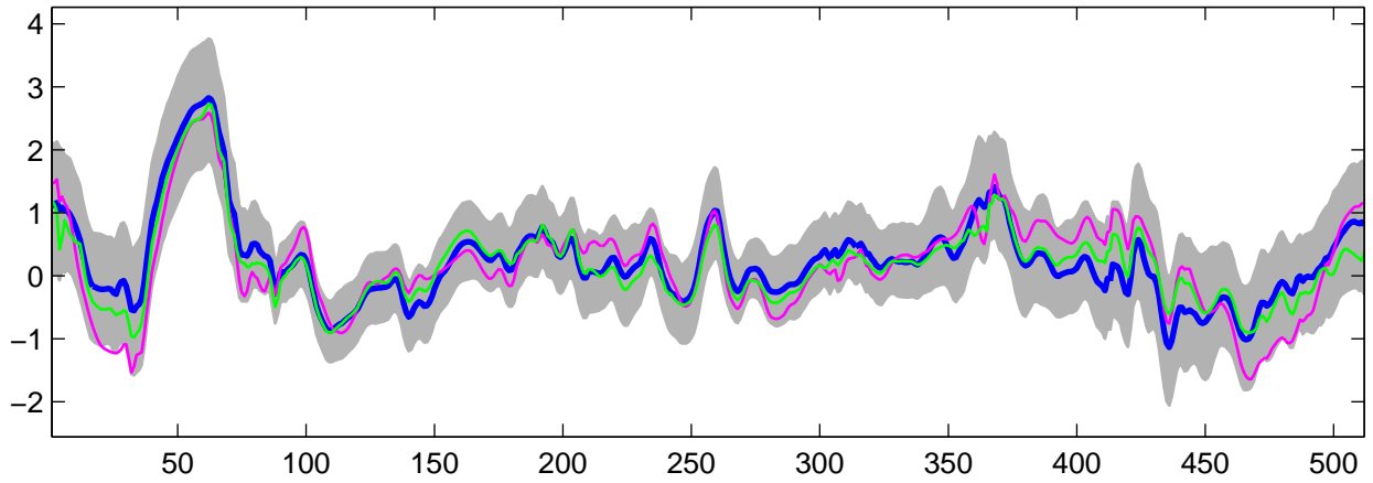
Estimated U_{21}(t) using G-WFMM: t_3 data, run 7
