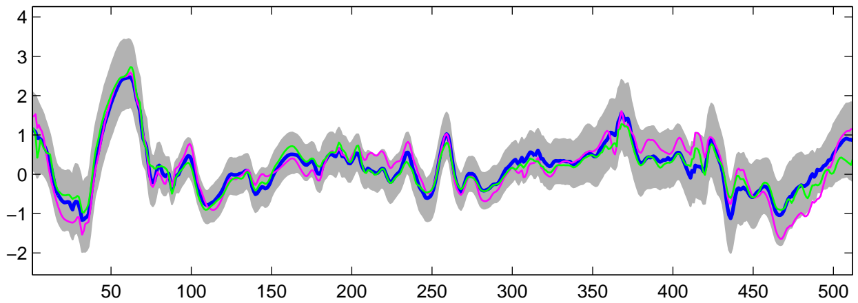
Estimated U_{21}(t) using R-WFMM: t_3 data, run 7
