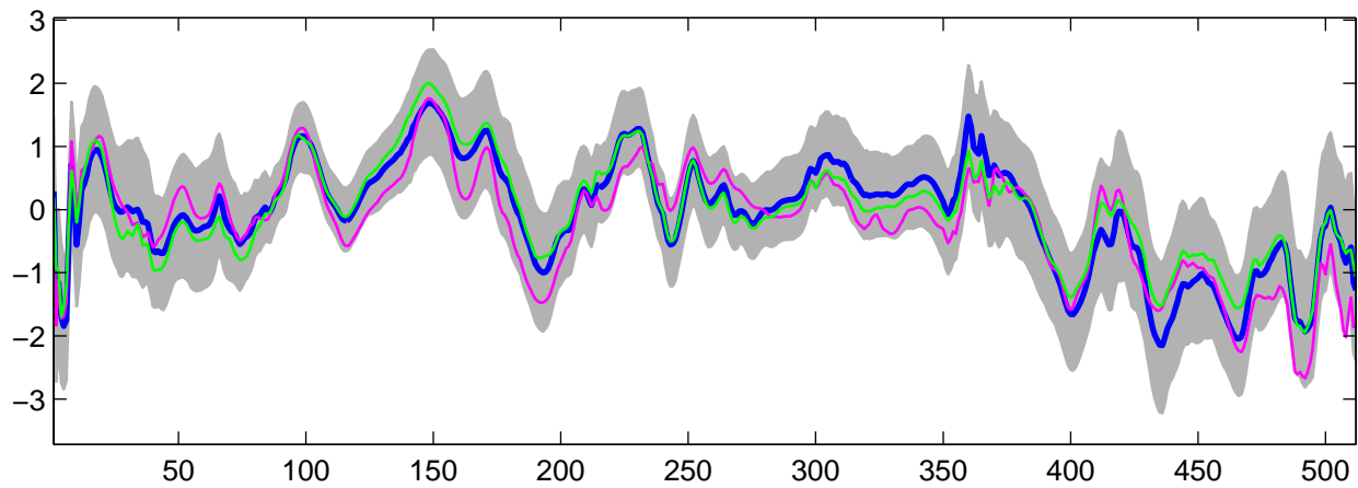
Estimated U_{22}(t) using G-WFMM: DE data, run 7
