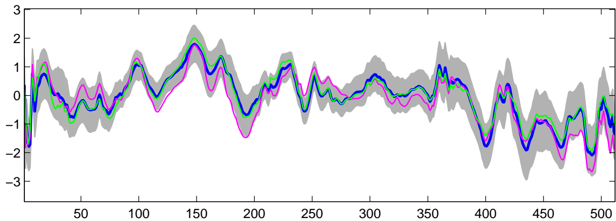
Estimated U_{22}(t) using R-WFMM: DE data, run 7
