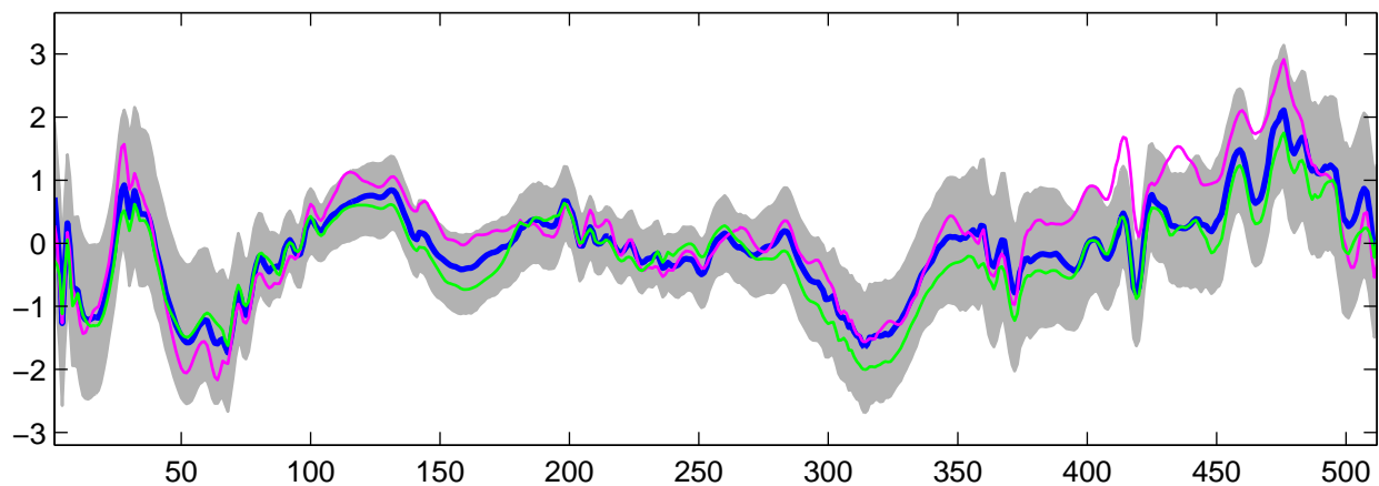
Estimated U_{22}(t) using R-WFMM: Normal data, run 7
