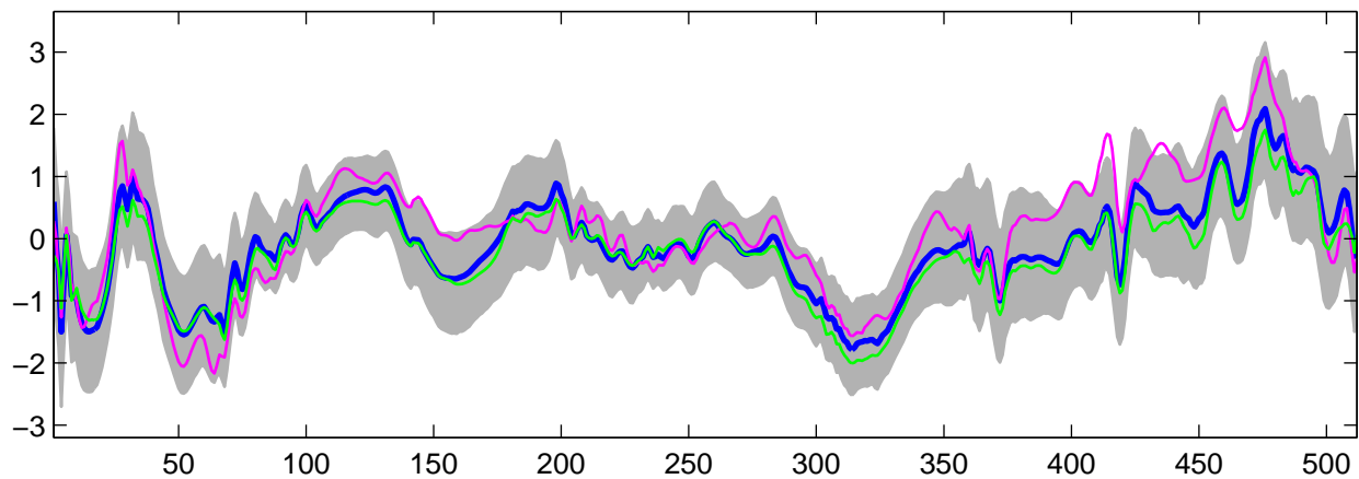
Estimated U_{22}(t) using G-WFMM: Normal data, run 7
